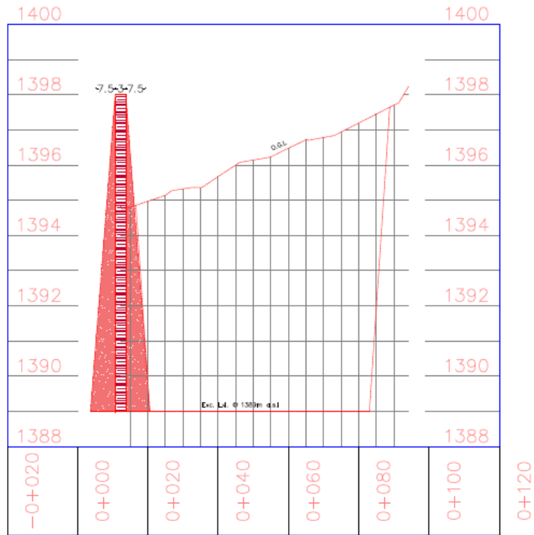
DAM FETCH PROFILE
