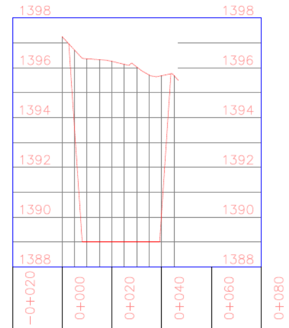
DAM X-X PROFILE
